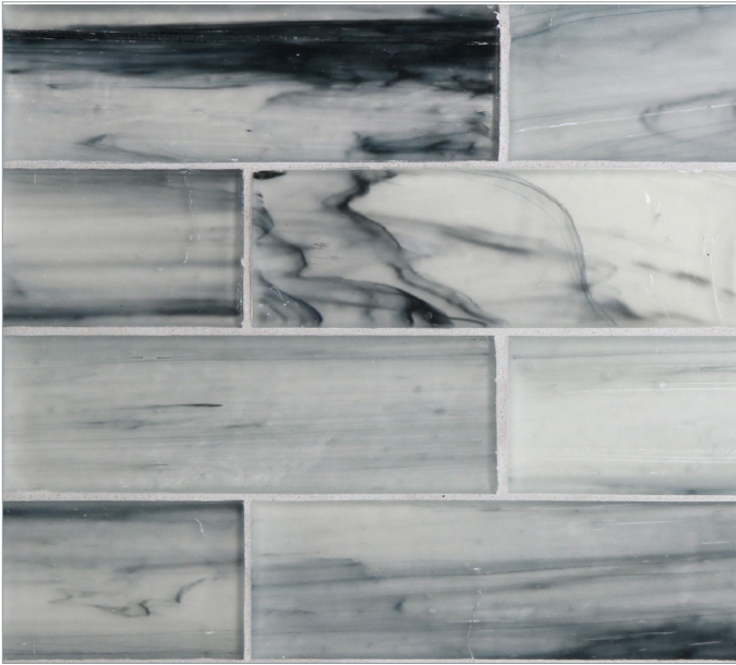
Argon Natural
