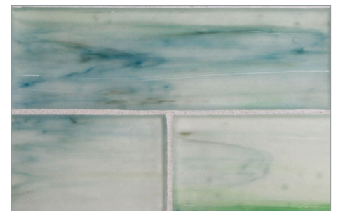
Erbium Natural
