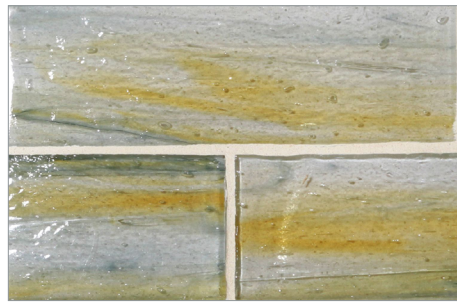
Xenon Natural
