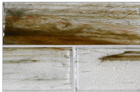
Strontium Natural
