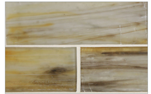
Yttrium Natural
