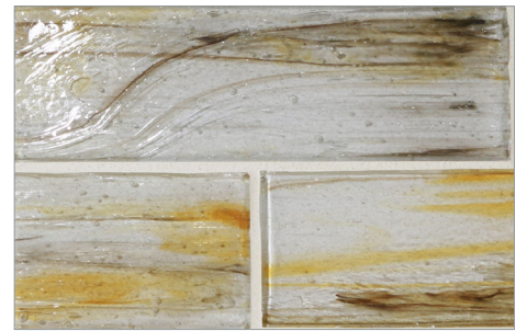
Tin Natural
