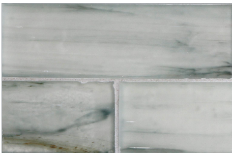
Oxygen Natural
