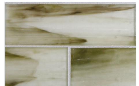
Selenium Natural
