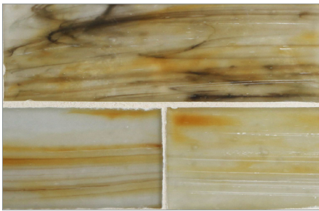
Tin Natural
